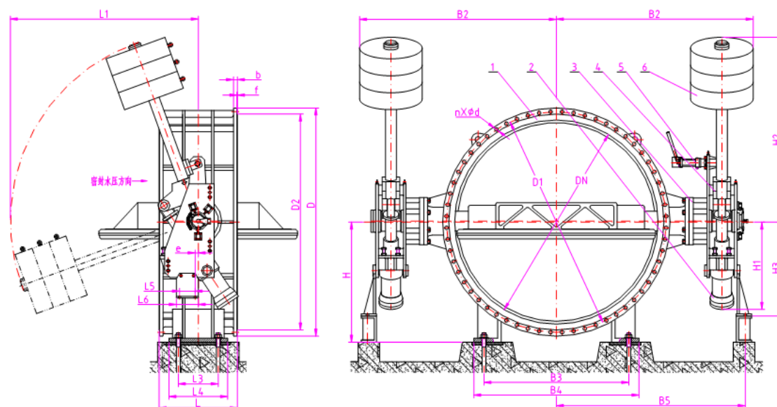
1、valve 2、Oil Cylinder 3、Transmission Support 4、Rocking Arm 5、Locking Oil Cylinder 6、Heavy Hammer 7、Release lever
